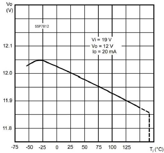
Figure 5: Output voltage vs Junction temperature
