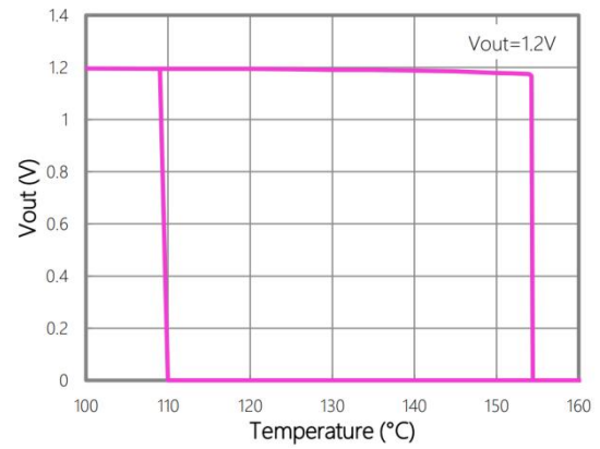
OTP Hysteresis
