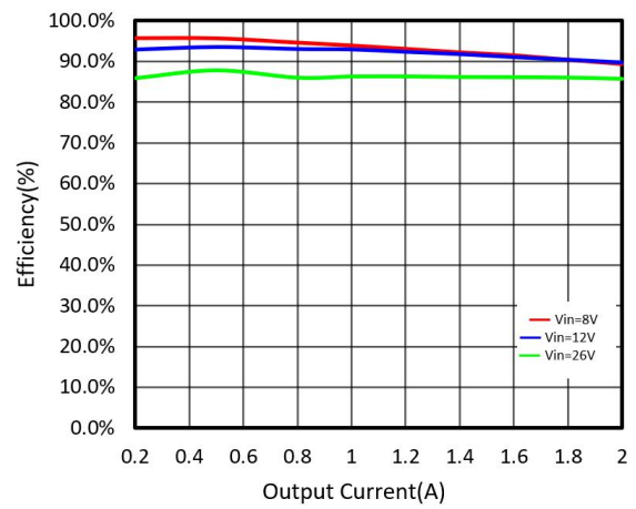
(8) efficiency and load current (output voltage 5.0V)
