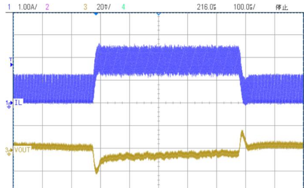
(16) Load transient (input voltage 15.0V, output voltage 5.0V, load current 0.5→1.8A)
