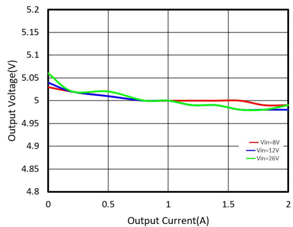
(4) Output Voltage and Load Current (Output Voltage 5.0V)
