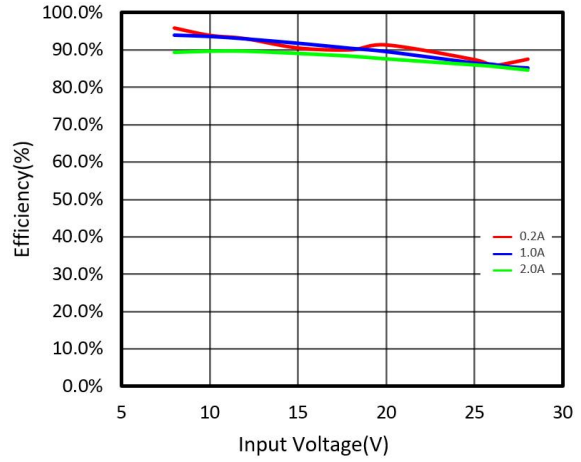
(10) efficiency and input voltage (output voltage 5.0V)
