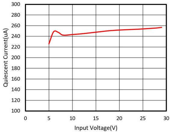
(1) Quiescent Current and Input Voltage
