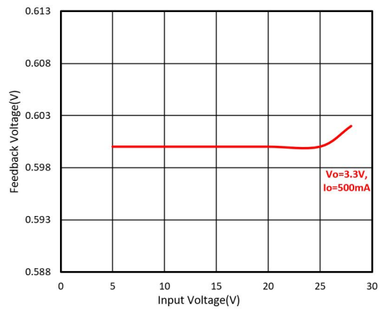
(2) Feedback Voltage and Input Voltage
