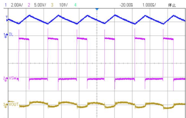
(14) Output ripple (input voltage 15.0V, output voltage 5.0V, load current 2A)
