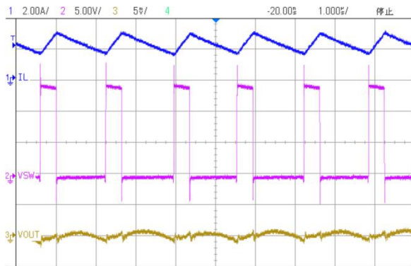
(13) Output ripple (input voltage 15.0V, output voltage 3.3V, load current 2A)
