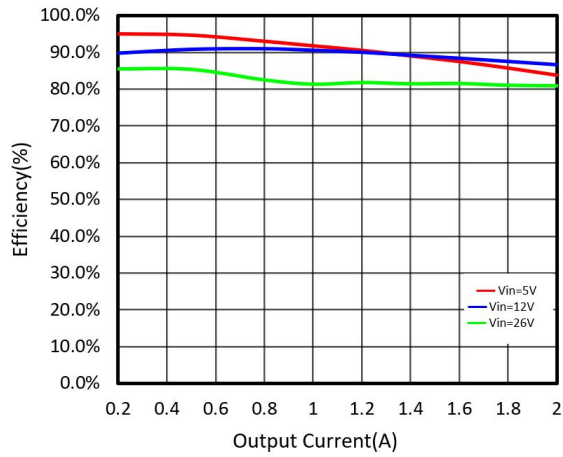
(7) efficiency and load current (output voltage 3.3V)
