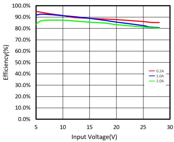
(9) efficiency and input voltage (output voltage 3.3V)
