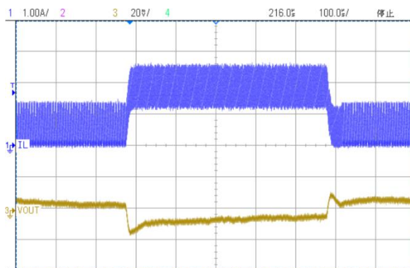
(15) Load transient (input voltage 15.0V, output voltage 3.3V, load current 0.5→1.8A)
